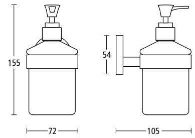
5550 Liquid soap dispenser. Finish: PC
