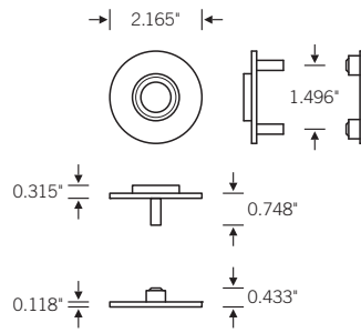
Flush Roses 0.118" (3 mm) × 2.165" (55 mm)
